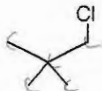
1-chloro-2,2-dimethylpropane
