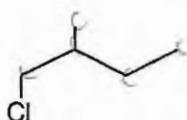
1-chloro-2-methylbutane
